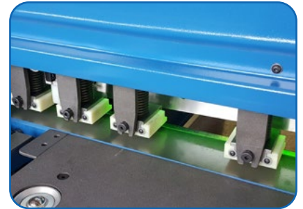
Specially-designed rectangular hold downs, suitable for cutting narrow stripes (optional)
