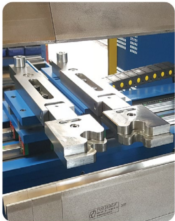
Specially designed finger stops offering high accuracy and maximum flexibility even in conical bends. Maximum stop position 1200mm.
